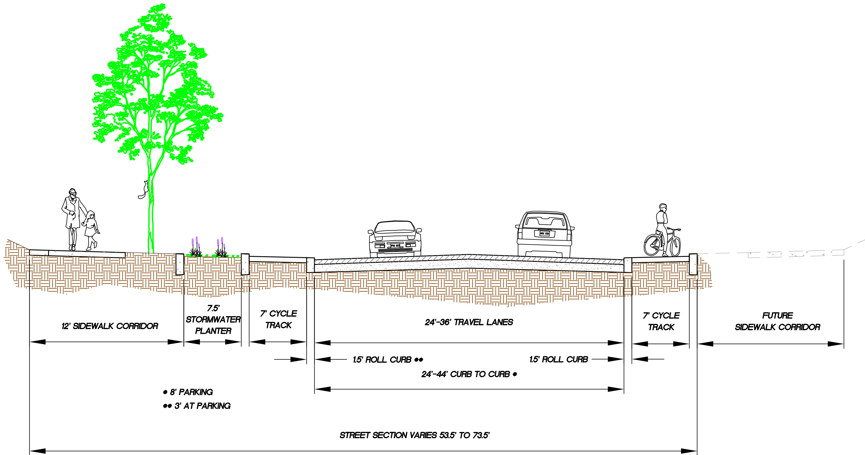
TYPICAL SECTION (LOOKING EAST)
