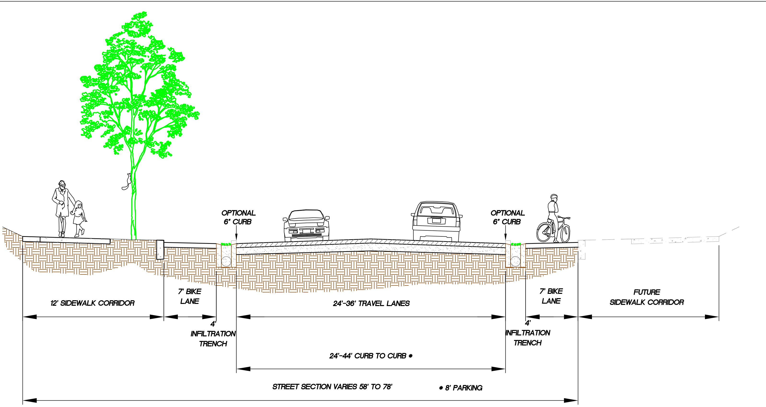
TYPICAL SECTION (LOOKING EAST)
