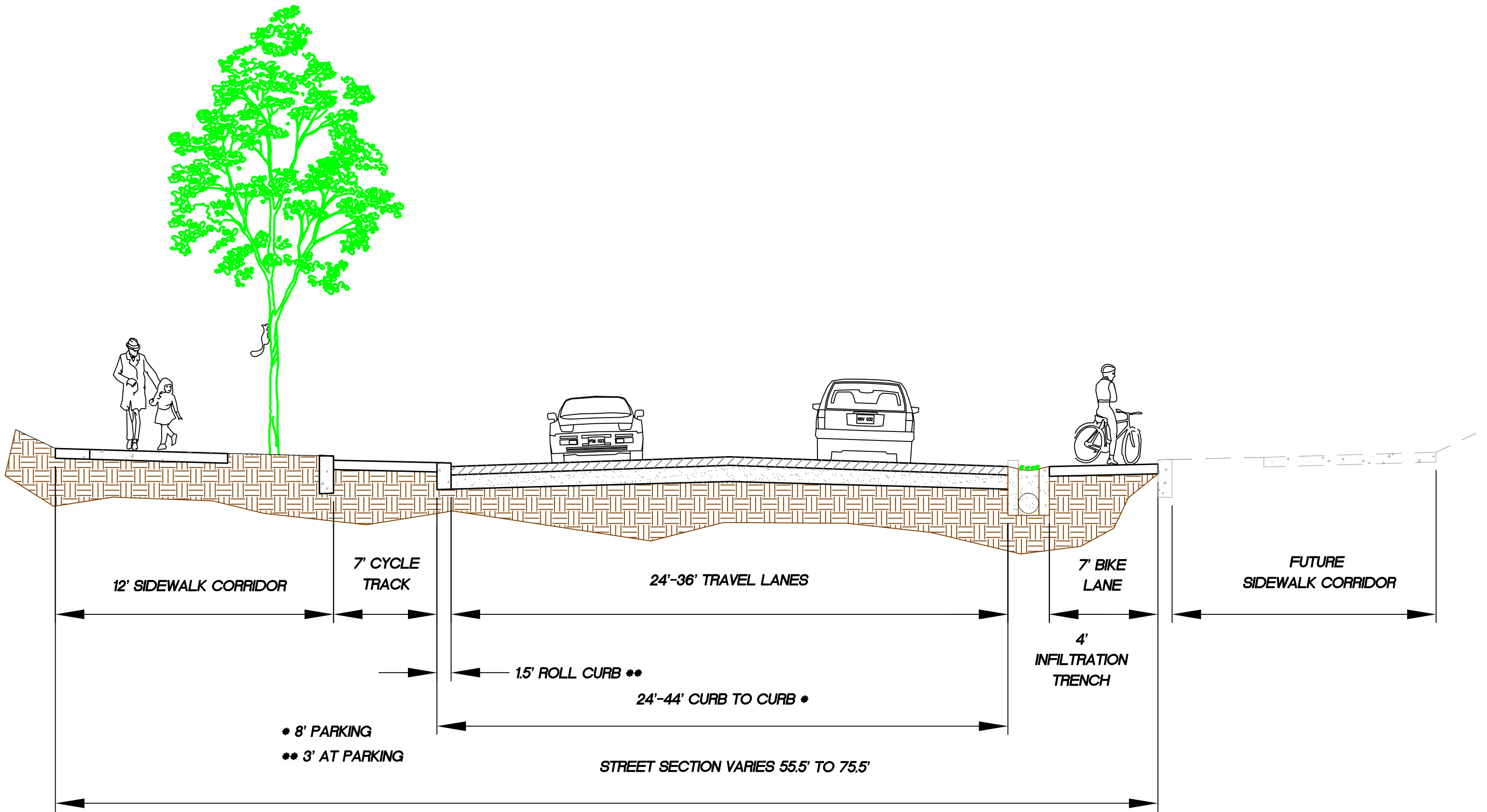
TYPICAL SECTION WITHOUT STORMWATER PLANTER (LOOKING EAST)
